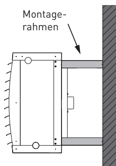
Abb. 4. Wandmontage
