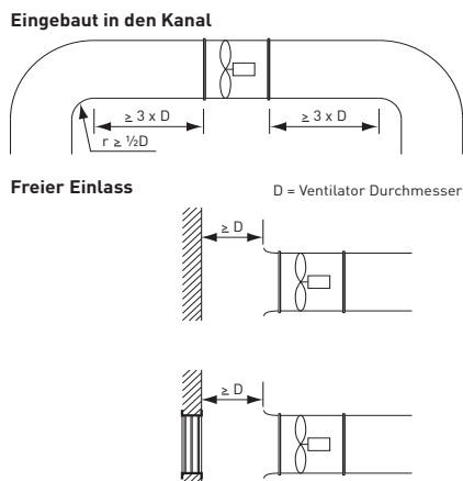
Fig. 9. Optimal Installation
