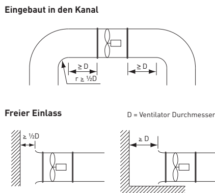
Fig. 10. Minimale Installation
