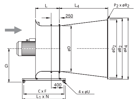
Support frame for ACG with long diffuser - hub sizes \phi 403 and \phi 578
