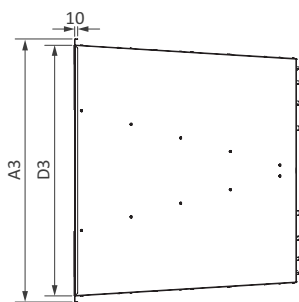
Round-to-square diffuser
