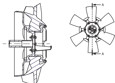
AZN 1000 impeller with Ø560 hub
