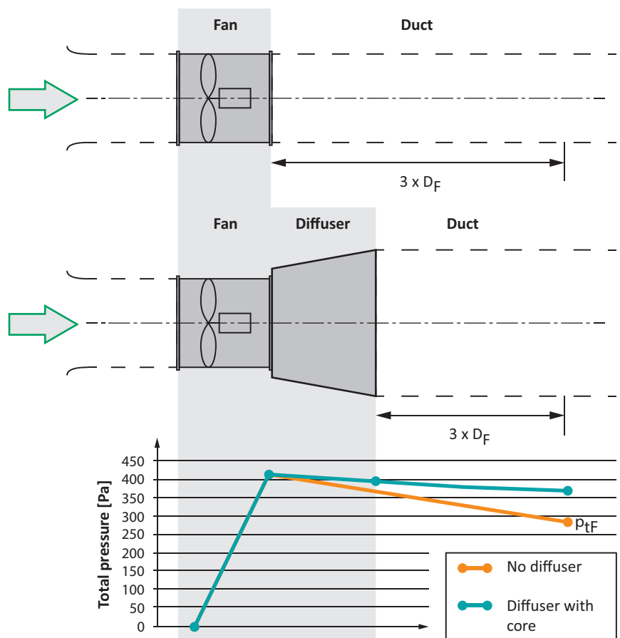
Pressure loss example
