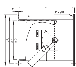
Damper type SBC
